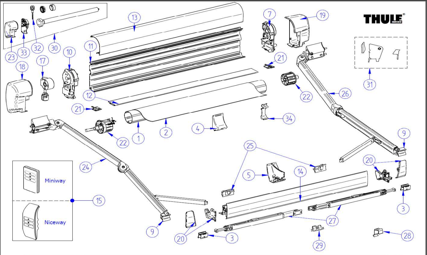
THULE Omnistor 8000
